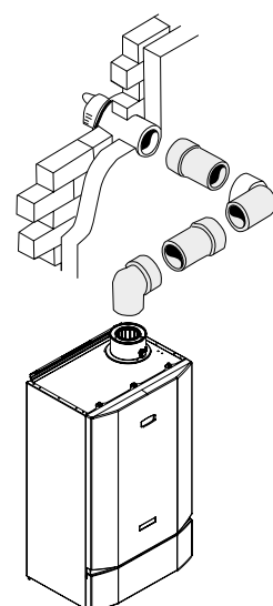
EXAMPLE 4 (CONCENTRIC)
