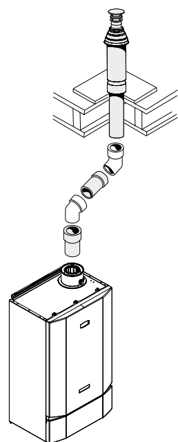
EXAMPLE 2 (CONCENTRIC)
