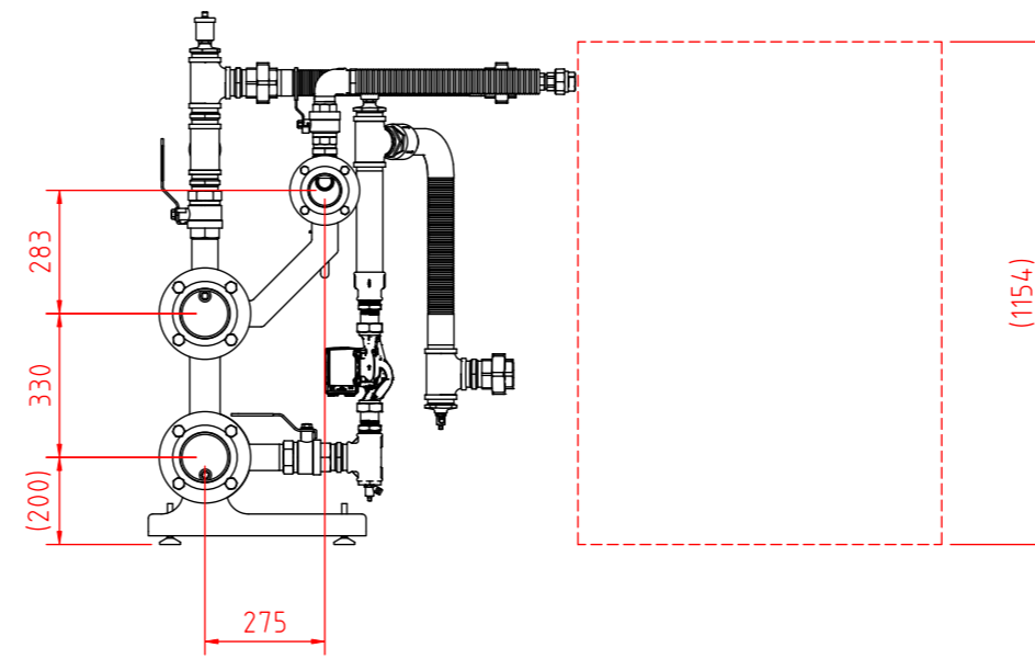
UIN 2264-06, IMAX XTRA 2, 4 BOILER HEADER KIT, 120-160kW, DN100 PN6 WATER, DN65 PN6 GAS, THREADED PUMP Ideal Heating reserves the right to amend details or specification without notice. If in doubt please contact an authorised representative
