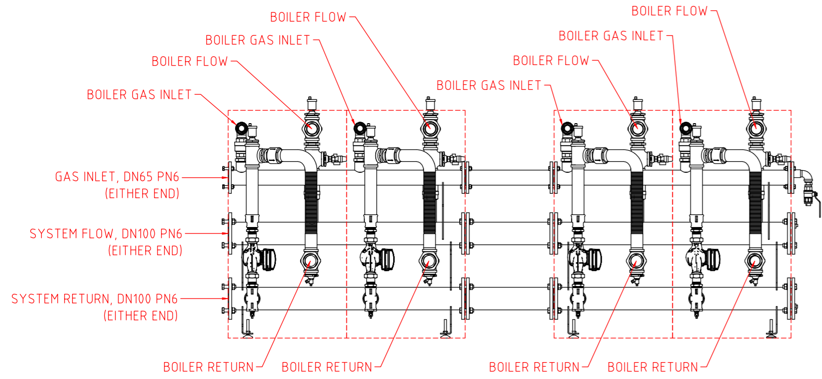
UIN 2264-06, IMAX XTRA 2, 4 BOILER HEADER KIT, 120-160kW, DN100 PN6 WATER, DN65 PN6 GAS, THREADED PUMP Ideal Heating reserves the right to amend details or specification without notice. If in doubt please contact an authorised representative
