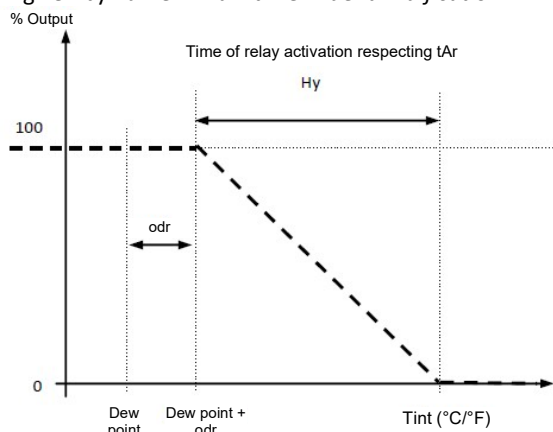
Figure 33: Dew point - Humidistat
