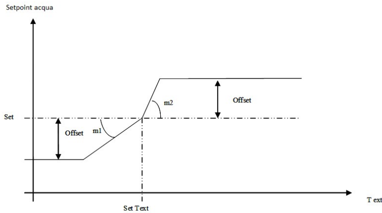
Figura 34. Chiller's climatic compensation
