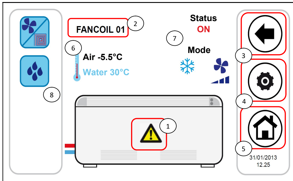
Figure 12. Information and fan coil page sensitive areas.
