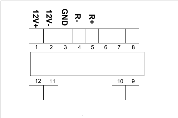
Figure 2. Connections.
